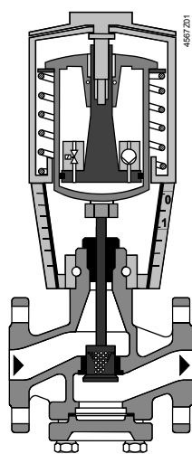
Valve closed
