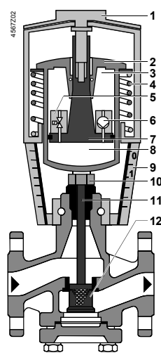
Valve open
